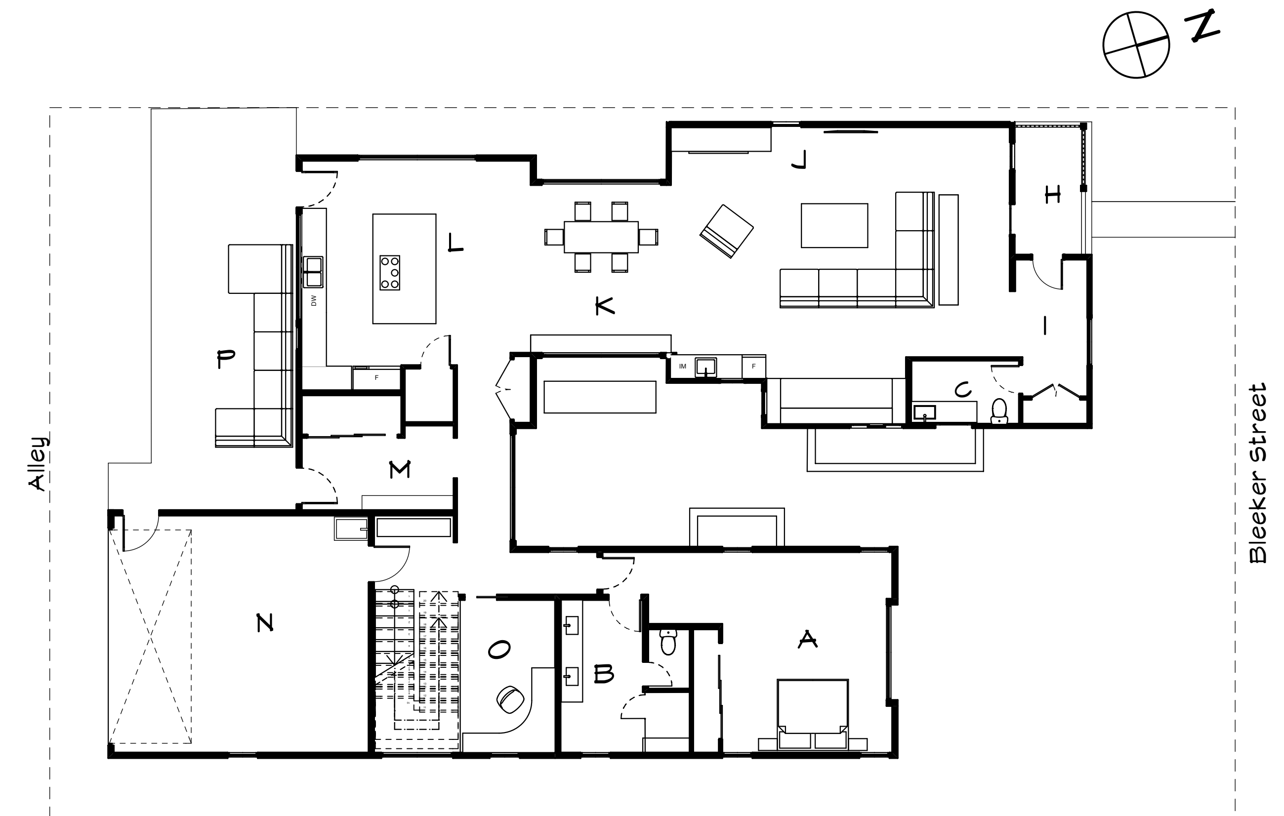
MAIN LEVEL PLAN
