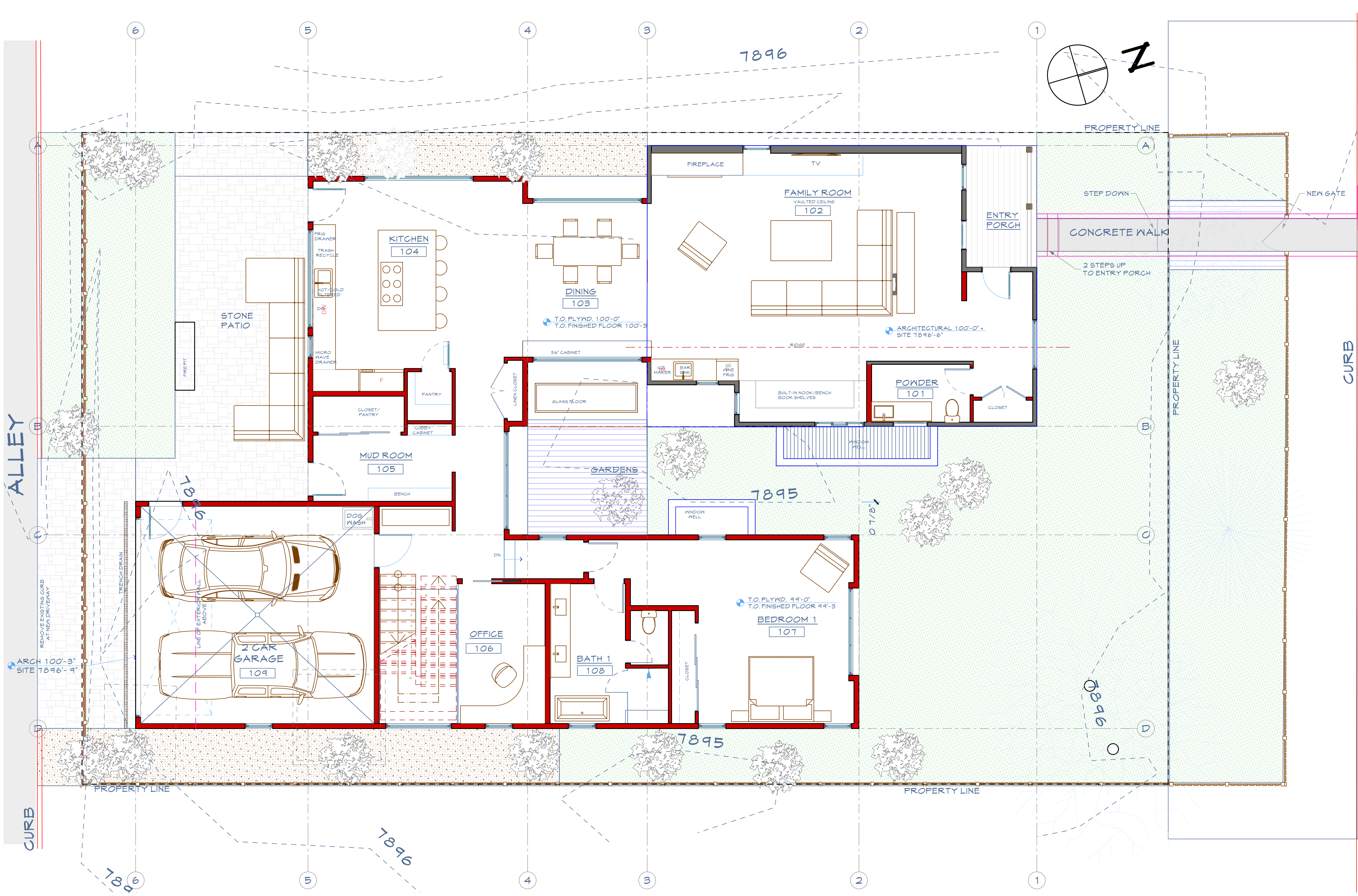
1 SITE PLAN A 1.0 SCALE: 1/4" = 1'-0"
